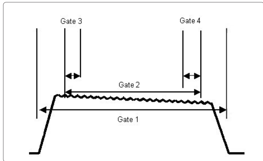
Figure 10 Powerful data configuration routines permit measurements during 4 gate times, each with 2 data “feeds” for display. Computed parameters such as peak-to-average ratio can also be displayed.
