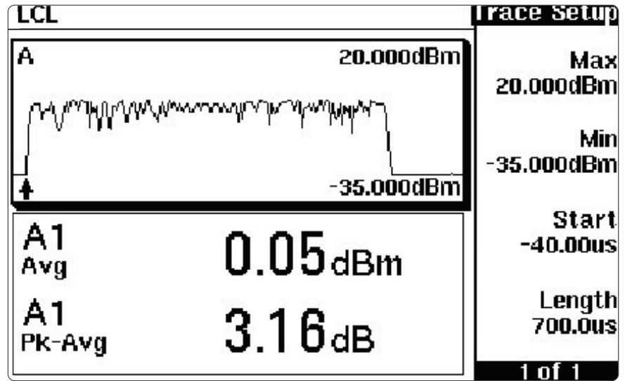
Figure 6 The display will show the EDGE data.
