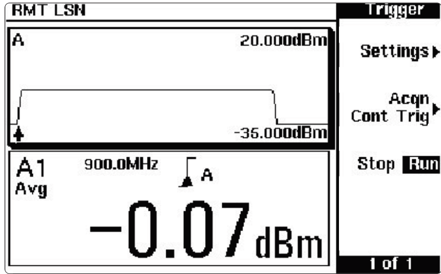
Figure 4 The display shows the GSM900 data
