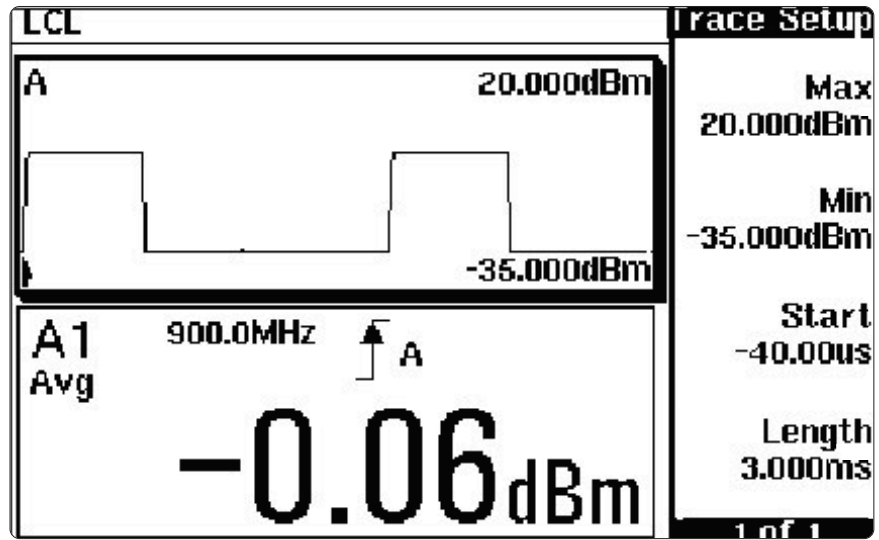
Figure 5 The display will show time slots 0 and 3 on (active)
