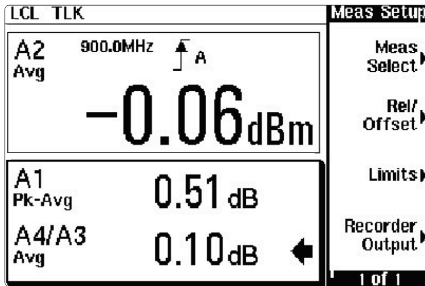
Figure 11 The display will now show the GSM900 data
