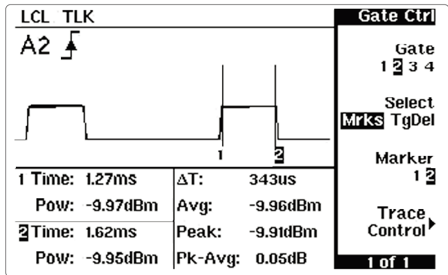
Figure 8 The display will show the following Bluetooth data
