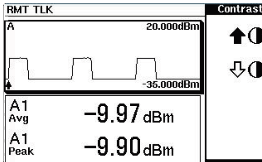
Figure 7 The display shows the Bluetooth data
