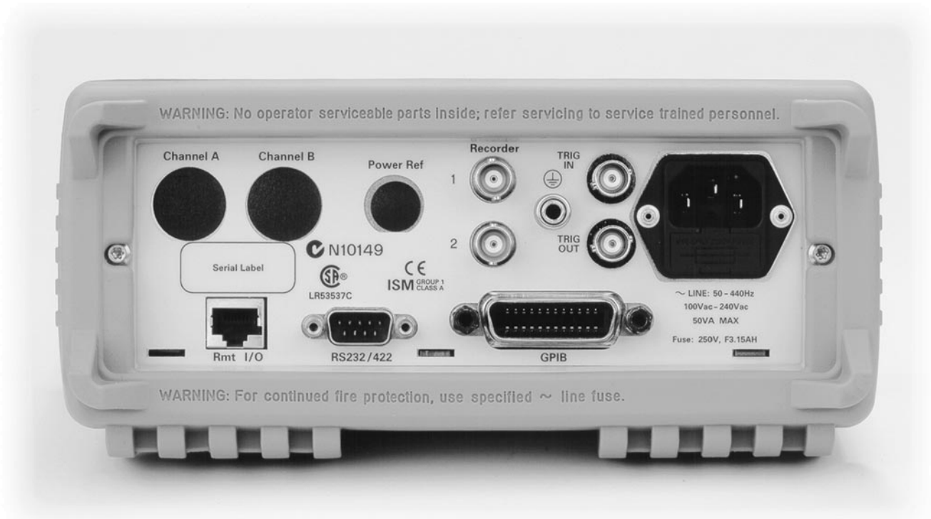
Figure 2. Rear Panel Overview
